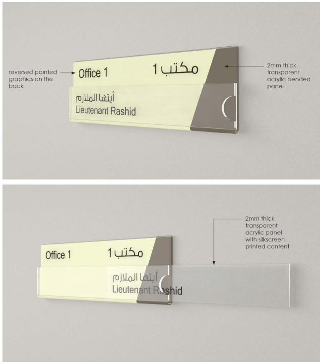
Design Elevation
